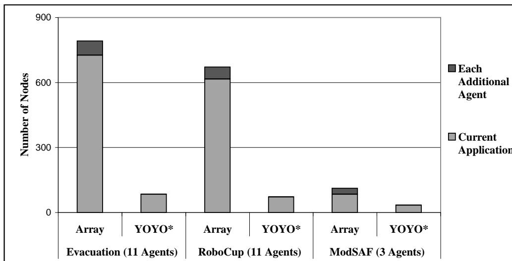
Figure 9: Empirical savings in applying YOYO* in the evacuation and other domains.
