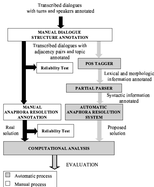
Figure 3: Full evaluation process
