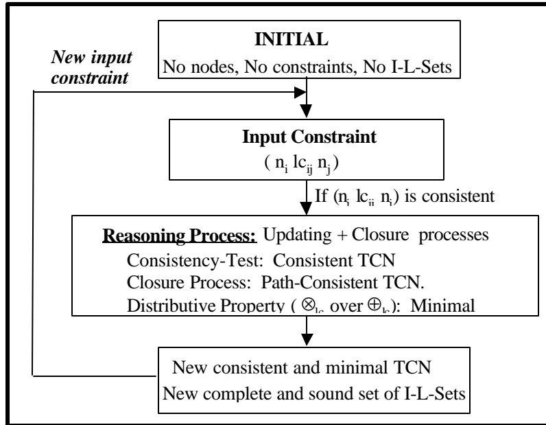
Figure 9: An incremental reasoning process
