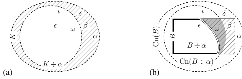
Figure 1: Building (b) base dependence via \text{Cond}^{\sim \rightarrow} is more complex than (a) dependence via \text{Cond}^{\sim \rightarrow} . Example formulas \alpha, \beta, \omega, \delta, \iota, \epsilon fall into different subareas. Assume K = Cn(B) .
