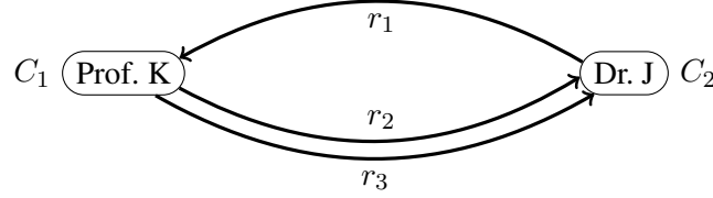
Figure 2: Contexts and bridge rules of the MCS M = (C_1, C_2) from Example 6.
