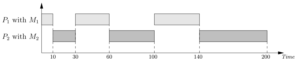
Figure 1: An example of the round-robin scheduling of PbP when running portfolio \{\langle P_1, M_1, \langle 10, 40, 160, \dots \rangle \rangle, \langle P_2, M_2, \langle 20, 60, 180, \dots \rangle \rangle\} on a given planning problem, assuming that planner P_1 using macros M_1 takes a total of 80 CPU-time units to terminate and P_2 with M_2 takes a total of 120 CPU-time units.
