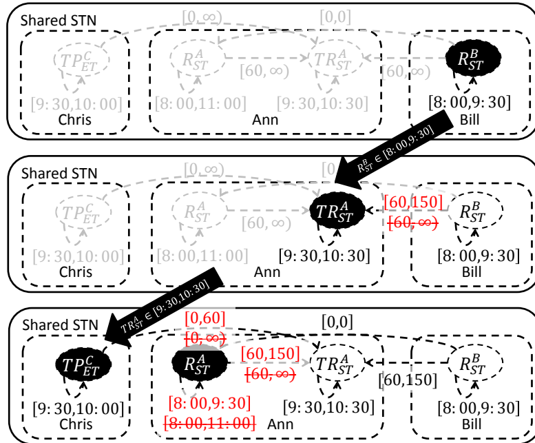
(b) As agents reinstate timepoints during the reverse sweep of the D\Delta PPC algorithm, each agent responds to each message it processed during the previous phase with updated edge information for that edge.
