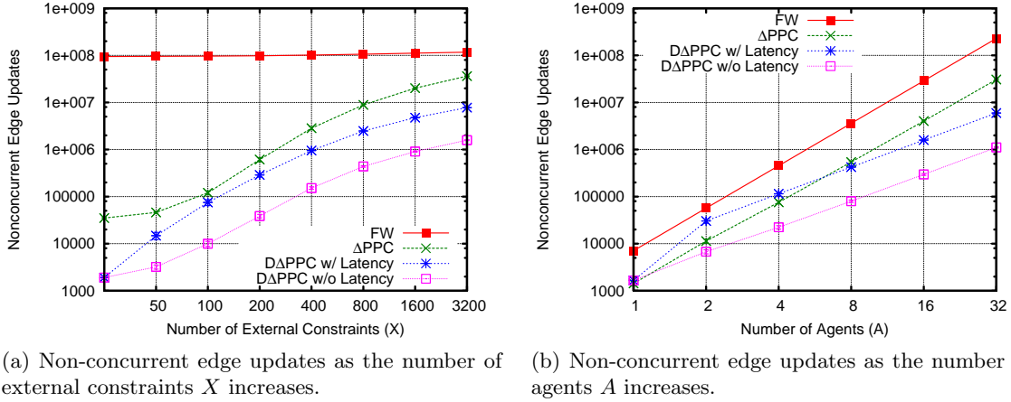
Figure 10: Empirical comparison of D \Delta PPC on the randomly generated problem set.
