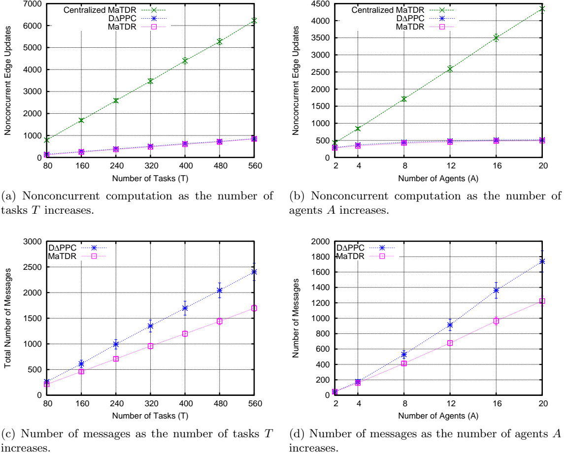
Figure 15: Empirical evaluation of MaTDR on the factory scheduling problem set.
