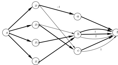
Figure 3: The flow network \text{SOFT\_ALLDIFFERENT}^{dec}() after projection
