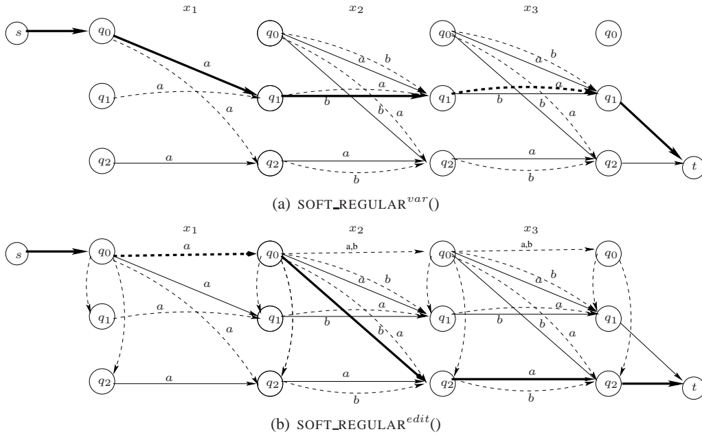
Figure 7: The flow network corresponding to the soft REGULAR constraints
