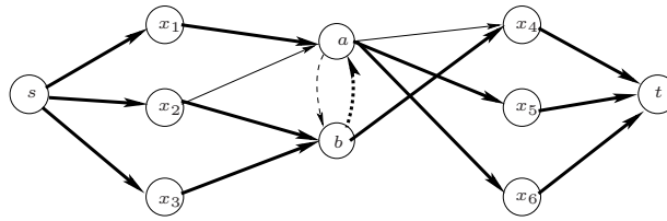
Figure 5: The flow network corresponding to the \text{SOFT\_SAME}^{\text{var}}(S_1, S_2) constraint
