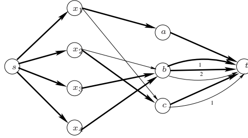
Figure 1: An example flow network for \text{SOFT\_ALLDIFFERENT}^{dec}
