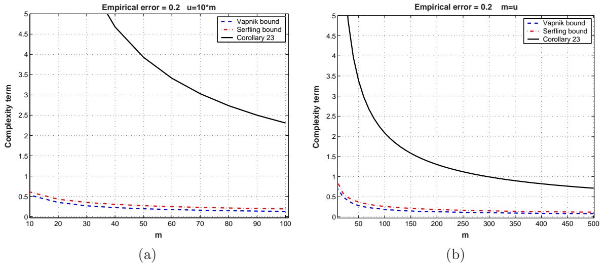
Figure 2: A comparison of Vapnik’s bound (Corollary 9), the bound of Theorem 22 (denoted here by “Serfling bound”) and the bound of Corollary 23. All bounds assume empirical error of 0.2, \delta = 0.01 and \mathbf{p}(h) = 1 . (a) u = 10m ; (b) u = m .
